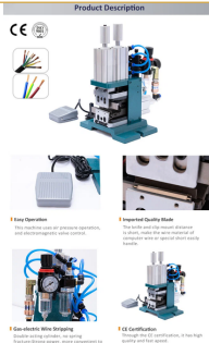
WPM-4F+T Automatic Multi-Core Wire Stripping & Twisting Machine
